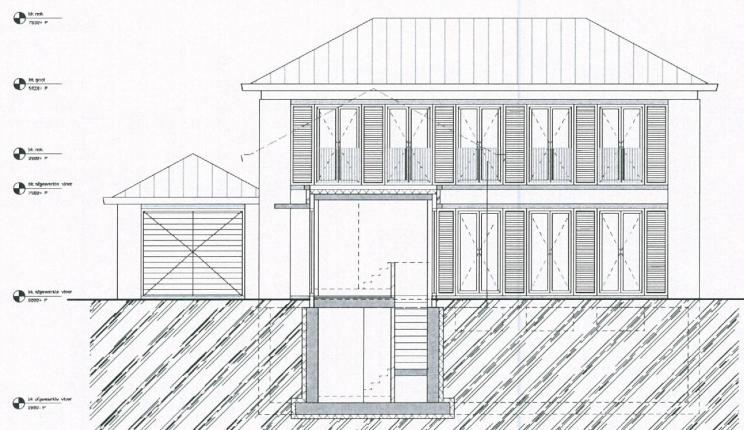
dwarsdoorsnede (A)
